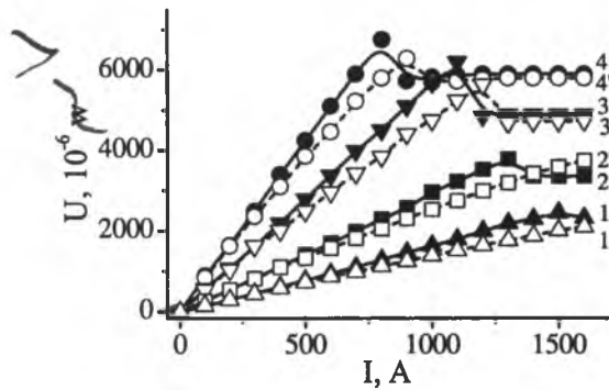
FIG. 3. Voltage along radius of a disk having hyperbolic section as a function of a current under external magnetic field B_0 , T: 3.5 (1, 1'); 4.9 (2, 2'); 7.1 (3, 3'); 8.4 (4, 4'); 1, 2, 3, 4 - collinear geometry of current flow, 1', 2', 3', 4' - anti-collinear geometry.
