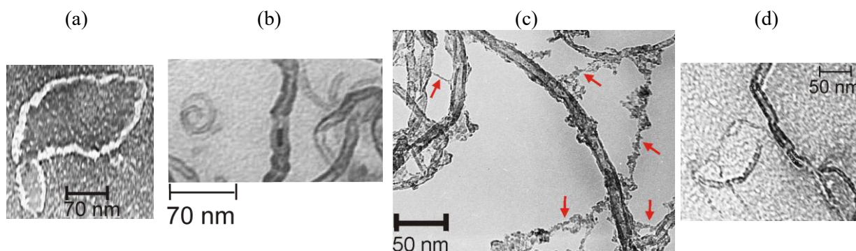
Figure 1. TEM-images of plasmid DNA molecules with different structure: (a) a native plasmid DNA; (b) a supercoiled cDNA in MWCNT-surroundings; (c) complexes ssDNA/MWCNT, arrows indicate denatured dsDNA molecules linking closely situated MWCNTs; (d) open circular ocDNA adhered to MWCNT.
